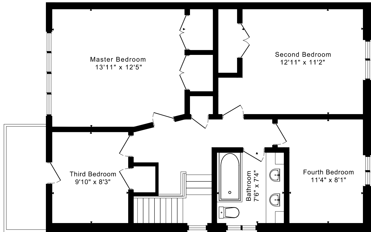
SECOND FLOOR 855 SQUARE FEET
